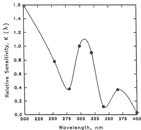
Fig. 3. Relative spectral sensitivity for B3 plastic film.
