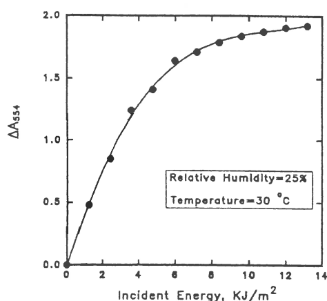
Fig. 9. Response of the B3 film to UV radiation emitted from the UVP ultraviolet crosslinker CL-1000. (Irradiance = 4 W/m 2 ).
